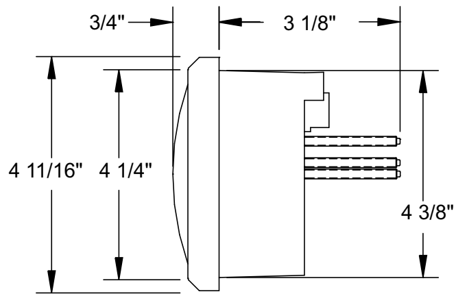
4 3/8" SPEEDOMETER
